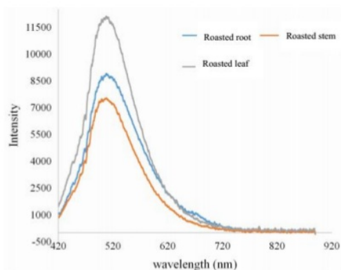
12 Figure 6. The Characterization Results of the Cdots by Roasting Technique using PL
