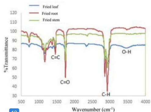
12 Figure 7. The Characterization Results of the Cdots by Frying Technique using FTIR
